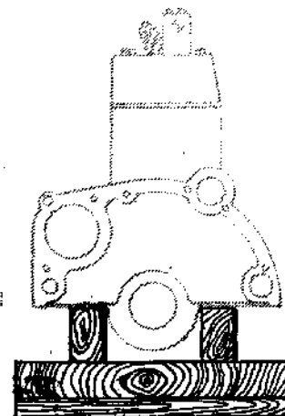
Fig. 4 - SUPPORT MR-3053-70
