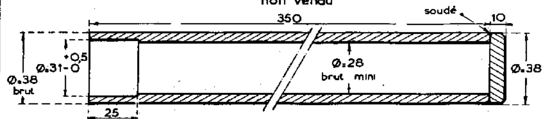
Fig 3 - MANDRIN MR-3045-10
